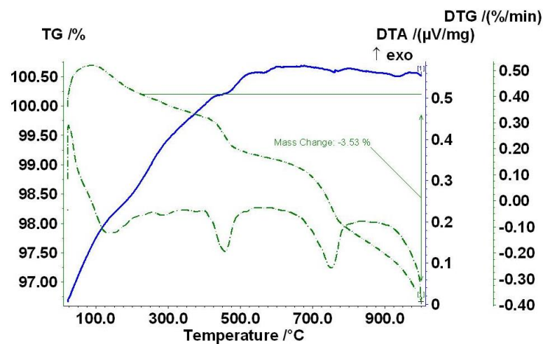
Figure 7. DTA/TG/DTG of fly ash "Stanari"
