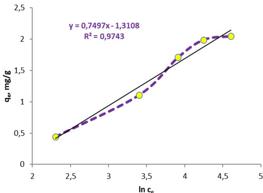
Figure 6. Temkin adsorption isotherm model for the system waste after shot blasting/ \text{Cu(II)} ions
