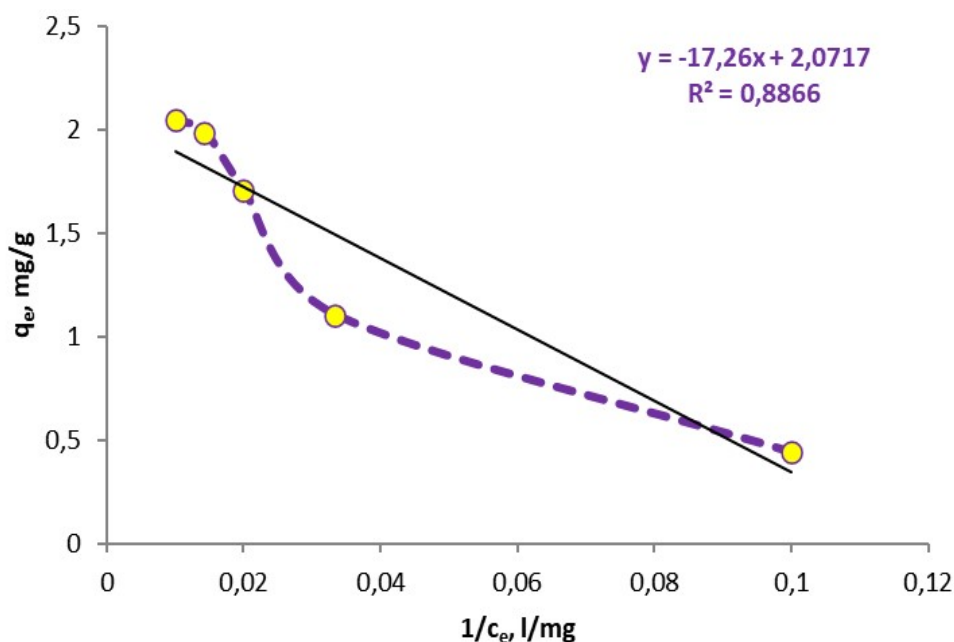
Figure 5. Eadie-Hoffstee adsorption isotherm model for the system waste after shot blasting/ \text{Cu(II)} ions
